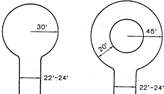
Circular turn arounds from Residential Streets, 2nd Edition .
