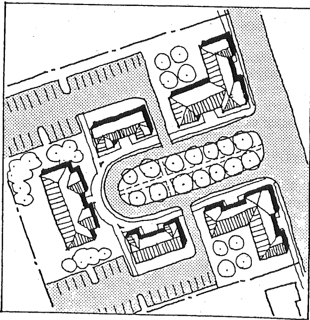
Preferred site planning which creates usable open space, adding value and identity to the complex, by siting parking behind the buildings.
